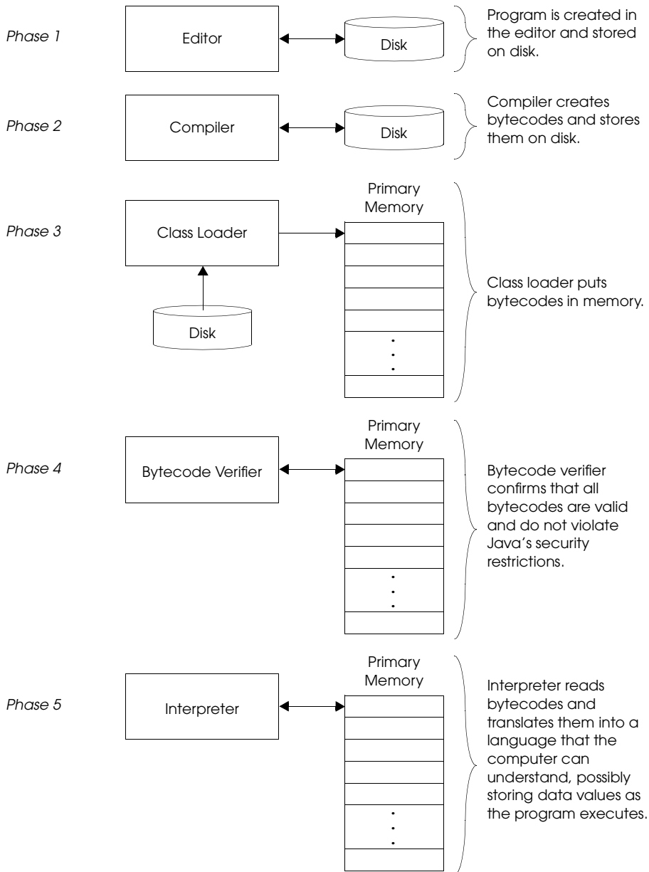
Fig. 1.1 A typical Java environment.
