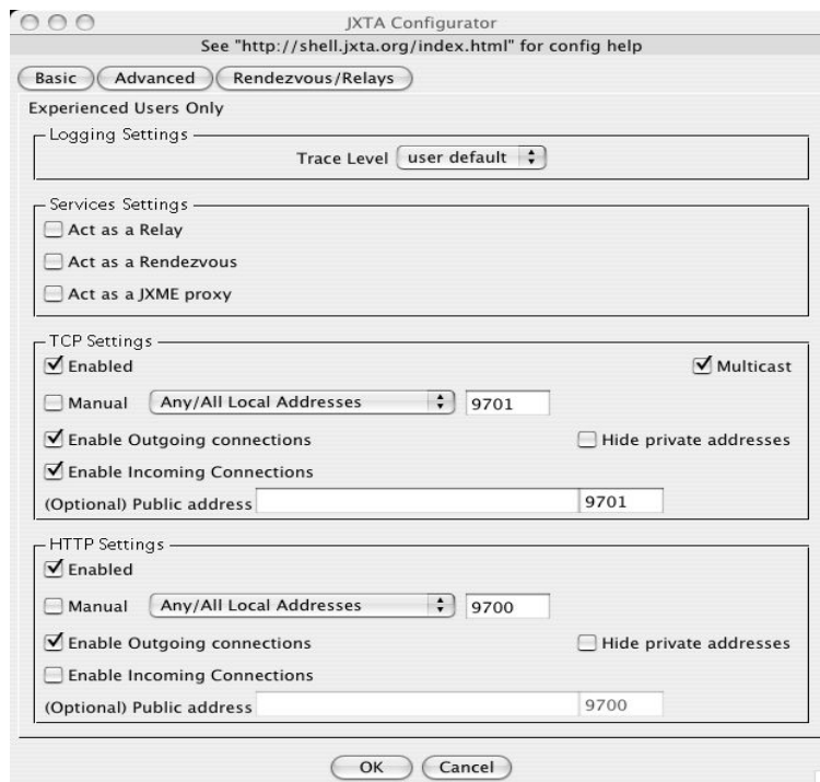
JXTA Configurator: Transport settings.
