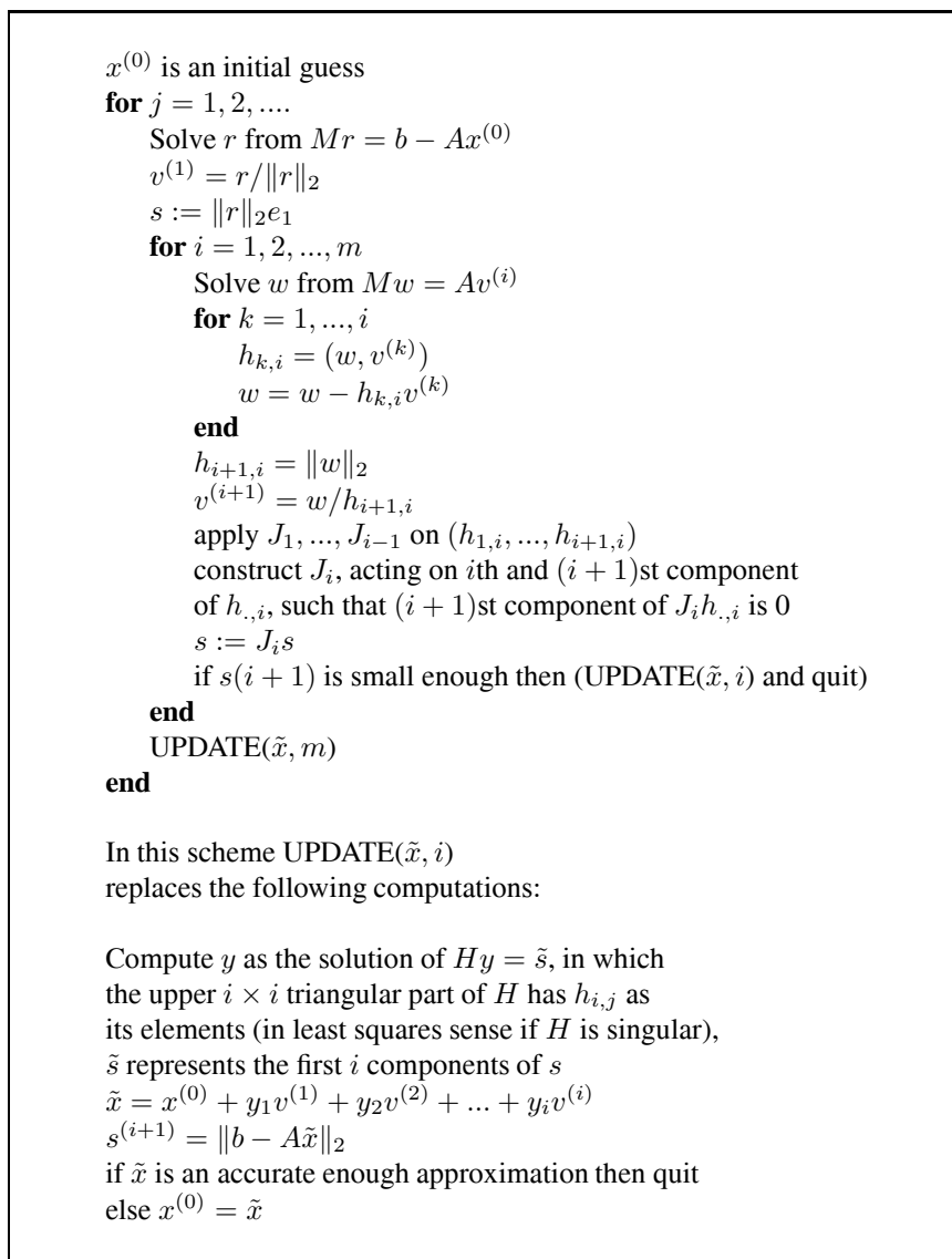
Figure 2.6: The Preconditioned GMRES( m ) Method
